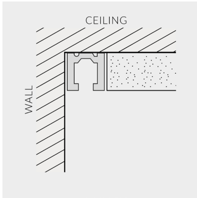
C TRACK Built into ceiling during construction or retrofit. Supports artworks up to 15kg each.
